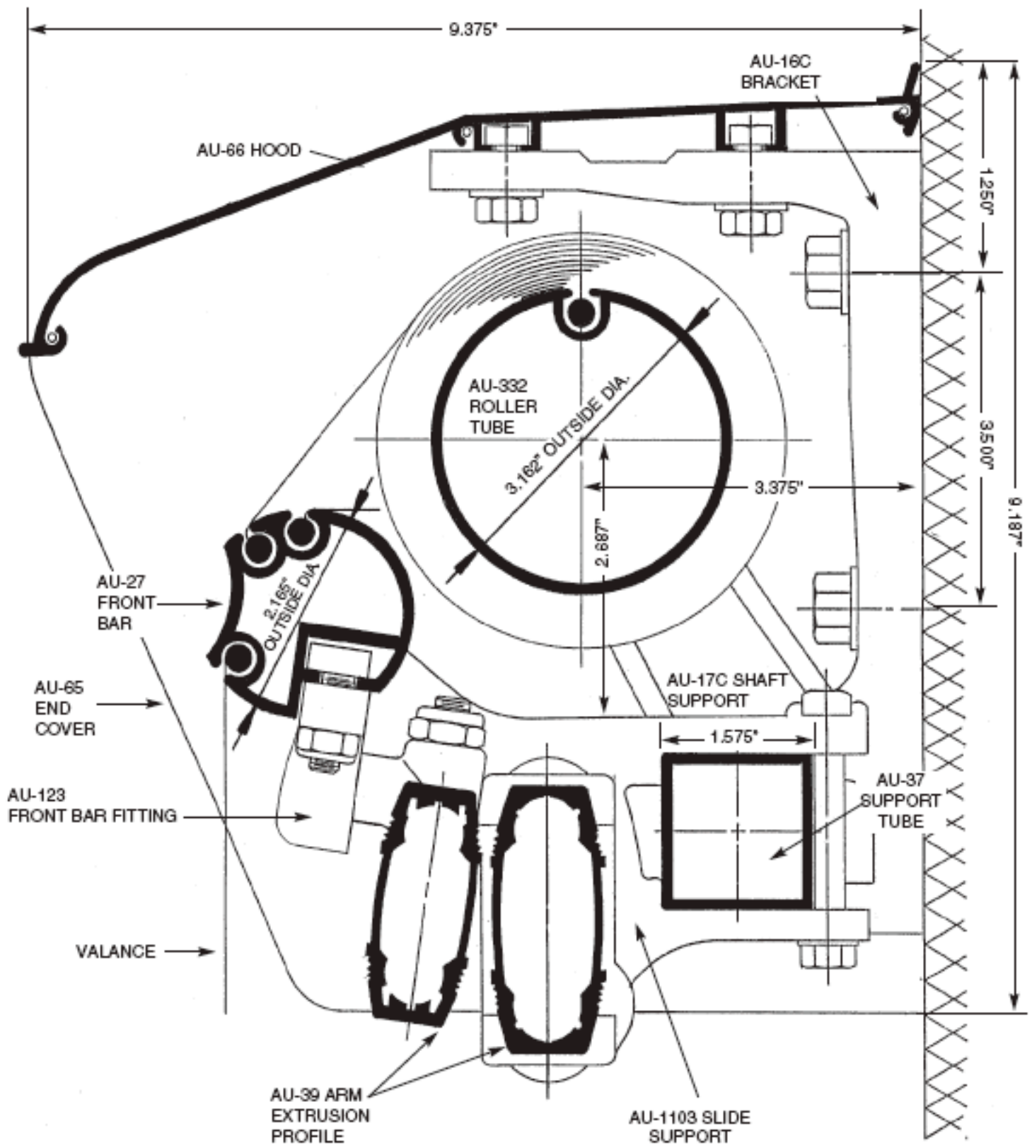
Cross section of Assembled Solair System in Retracted Position
